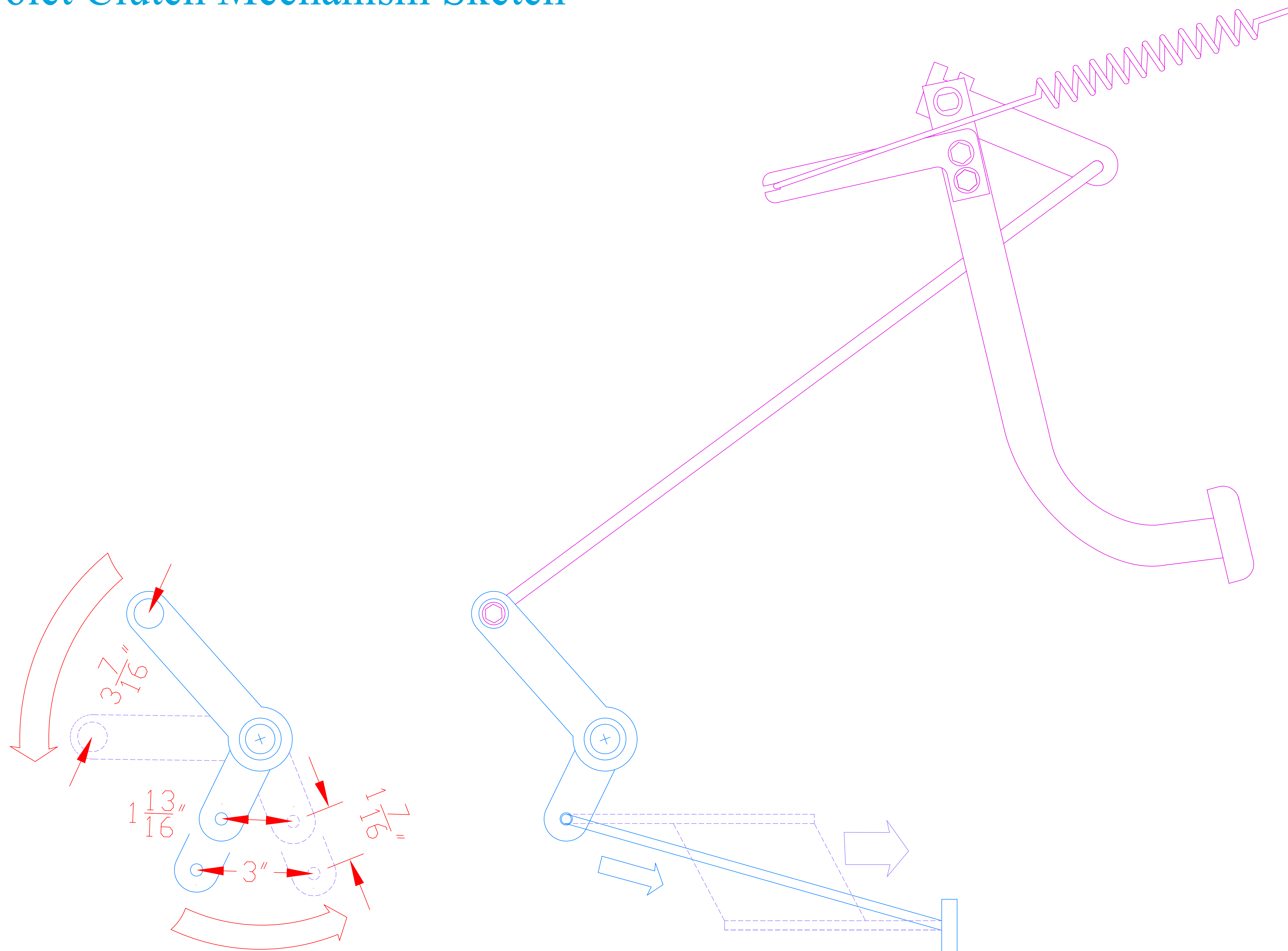
MODIFICATION OF CLUTCH CROSS SHAFT BY EXTENDING LOWER BAR -- SHOWS INCREASE IN TRAVEL. (DIMENSIONS SHOWN ARE TO SCALE BUT FOR REFERENCE ONLY)
